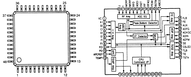
CXA1981 (IC101)
