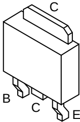
2SB1205 2SC4681
