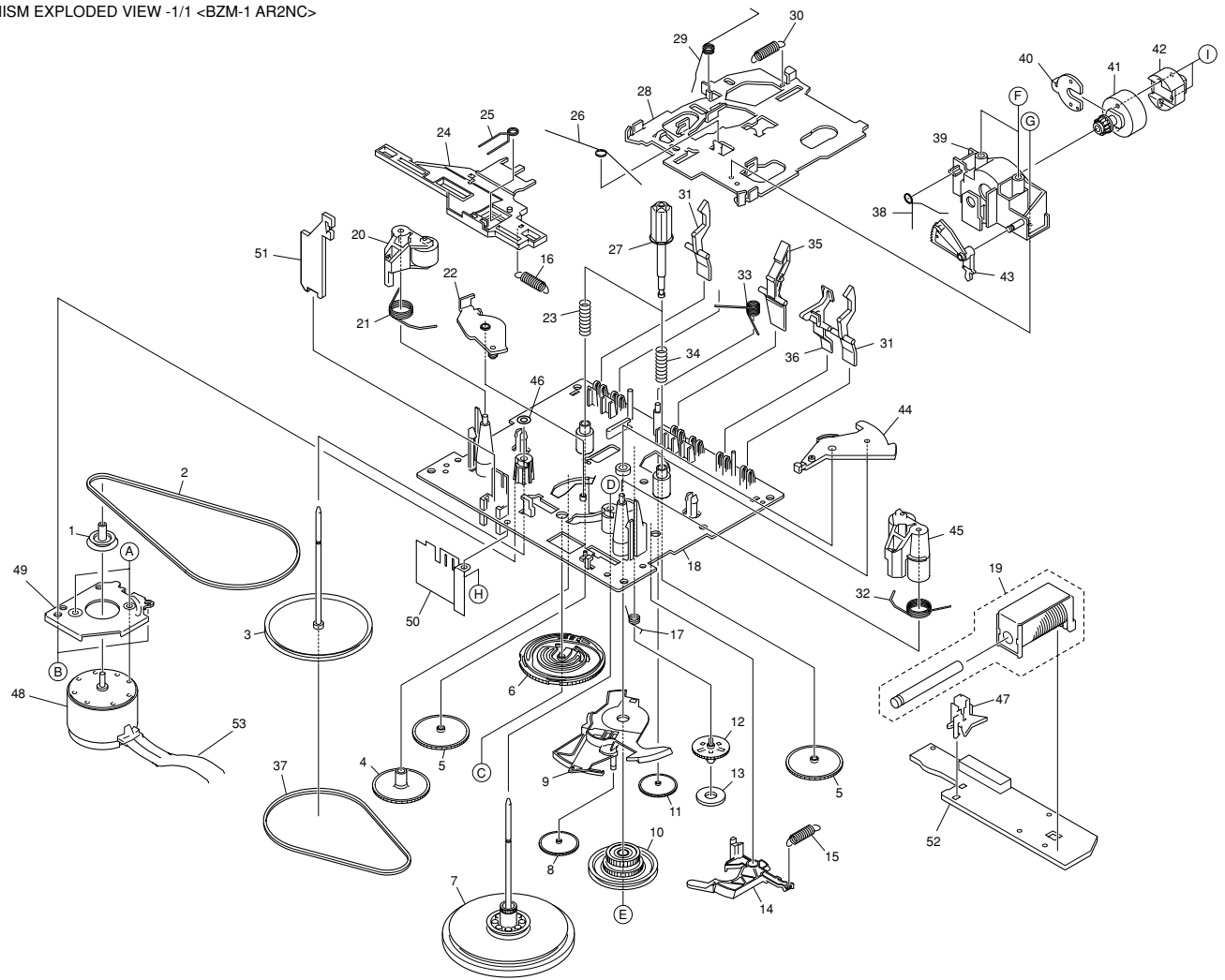
TAPE MECHANISM EXPLODED VIEW -1/1 <BZM-1 AR2NC>
