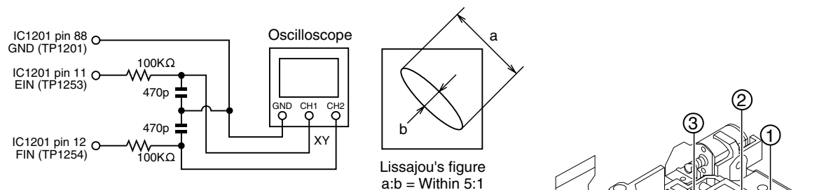
Fig. 14-1 Optical Pickup Grating Drift Measurement Method
