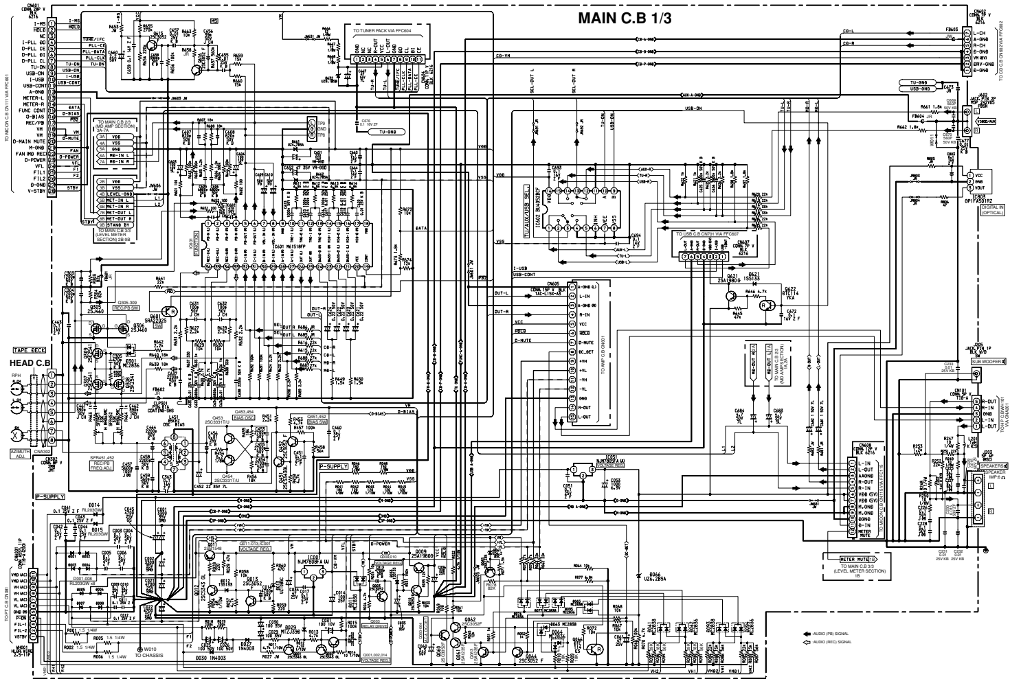
SCHEMATIC DIAGRAM - 1/10 (MAIN -1/3 SECTION)
