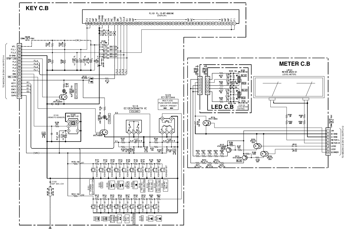
SCHEMATIC DIAGRAM - 8/10 (KEY/METER/LED SECTION)
