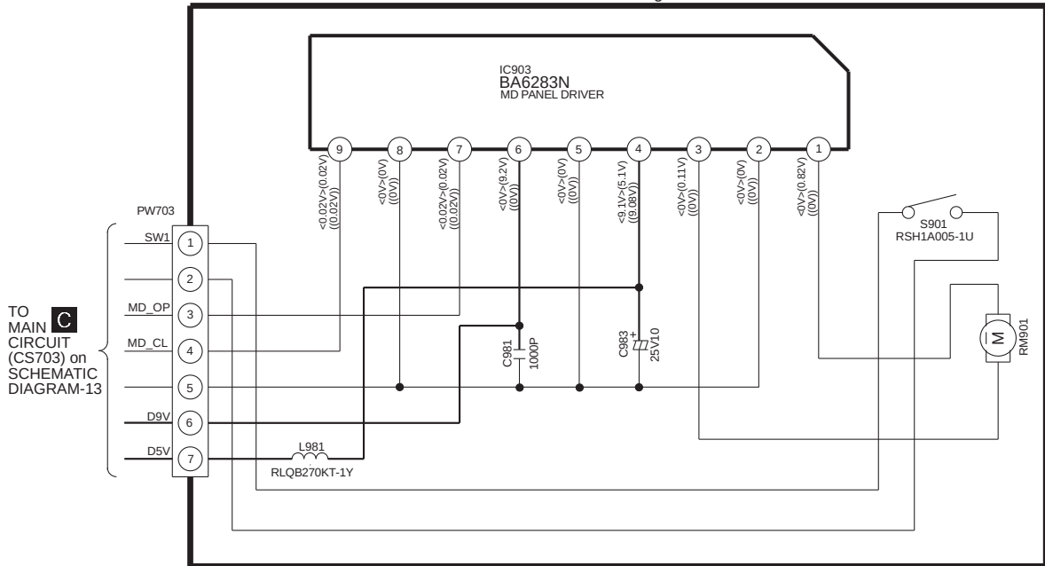
SCHEMATIC DIAGRAM-16
