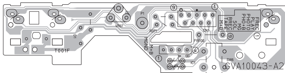
(Switch board)
