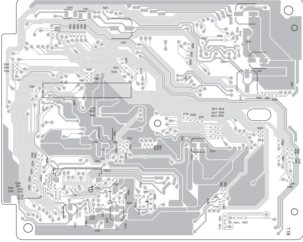
Reverse side
