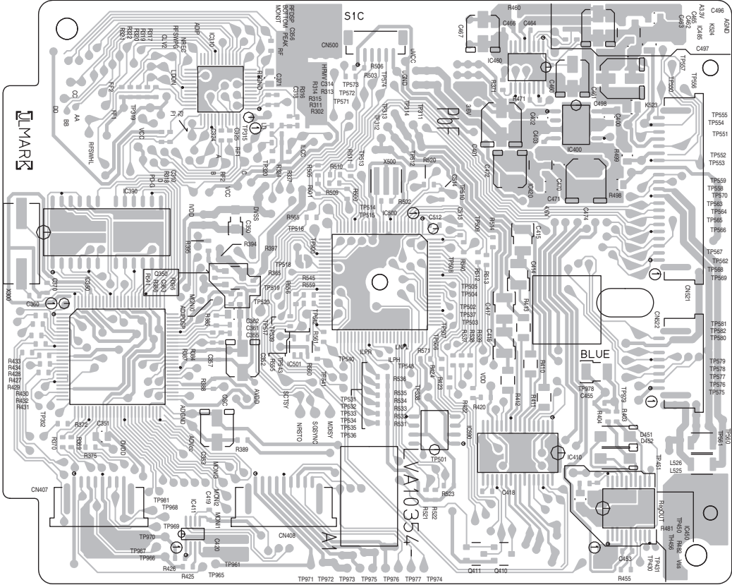
Reverse side
