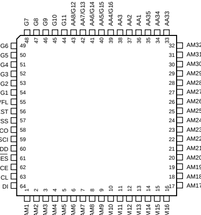
IC601 : LC75710NE FL Driver
