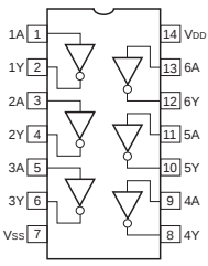
IC706 : TC74VHC04F Hex Inverters
