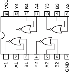
IC702 : HD74HC02FPEL Quad 2 Input NOR
