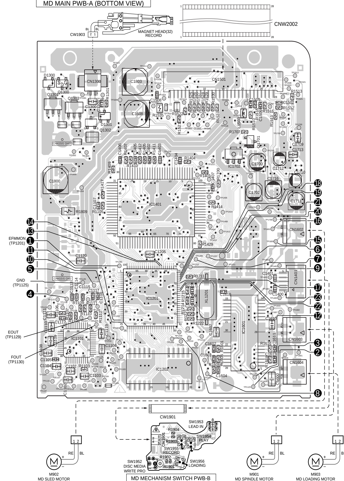
MD MAIN PWB-A (BOTTOM VIEW)
