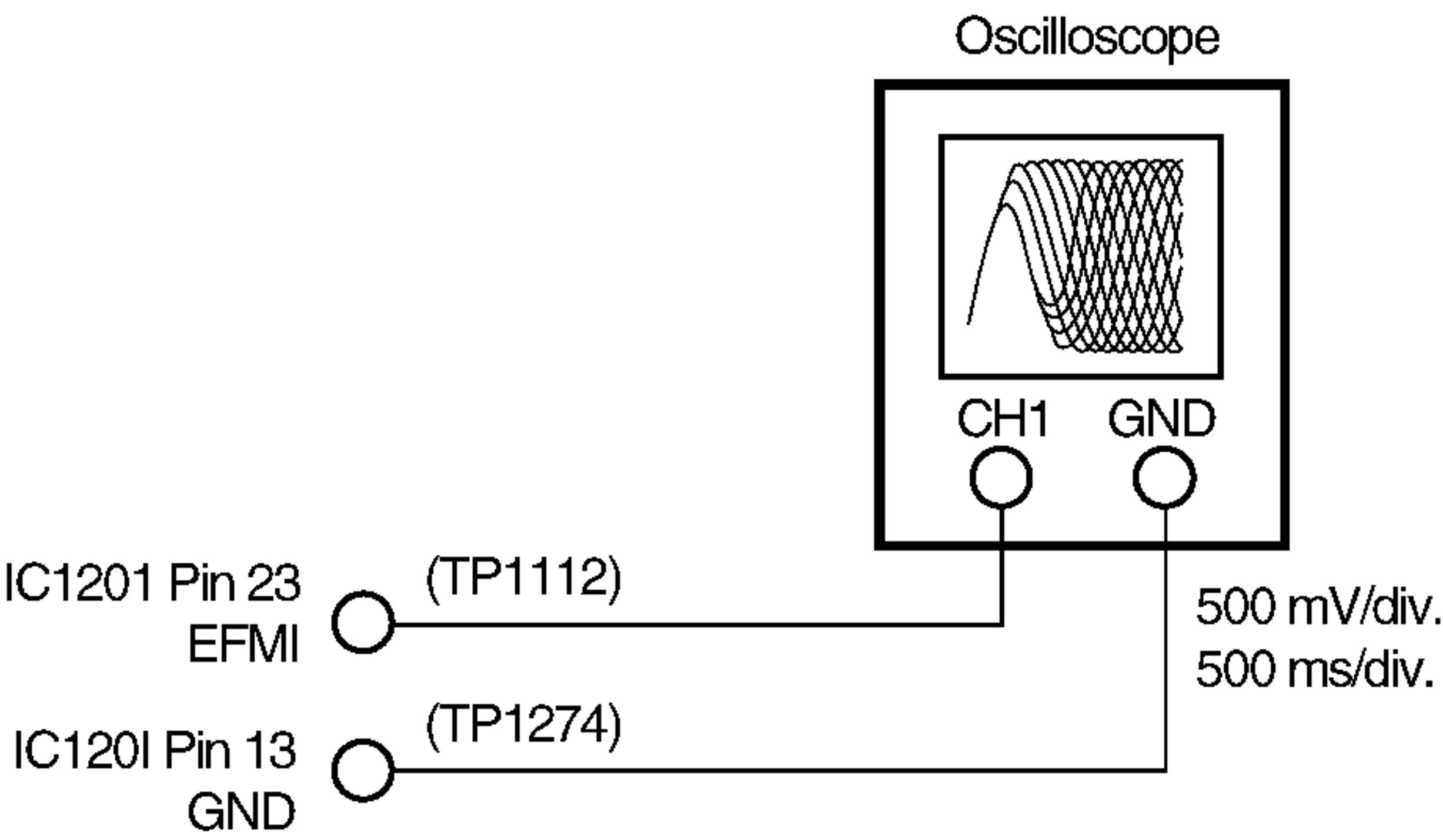
Fig. 6-7 Jitter Connection Diagram
