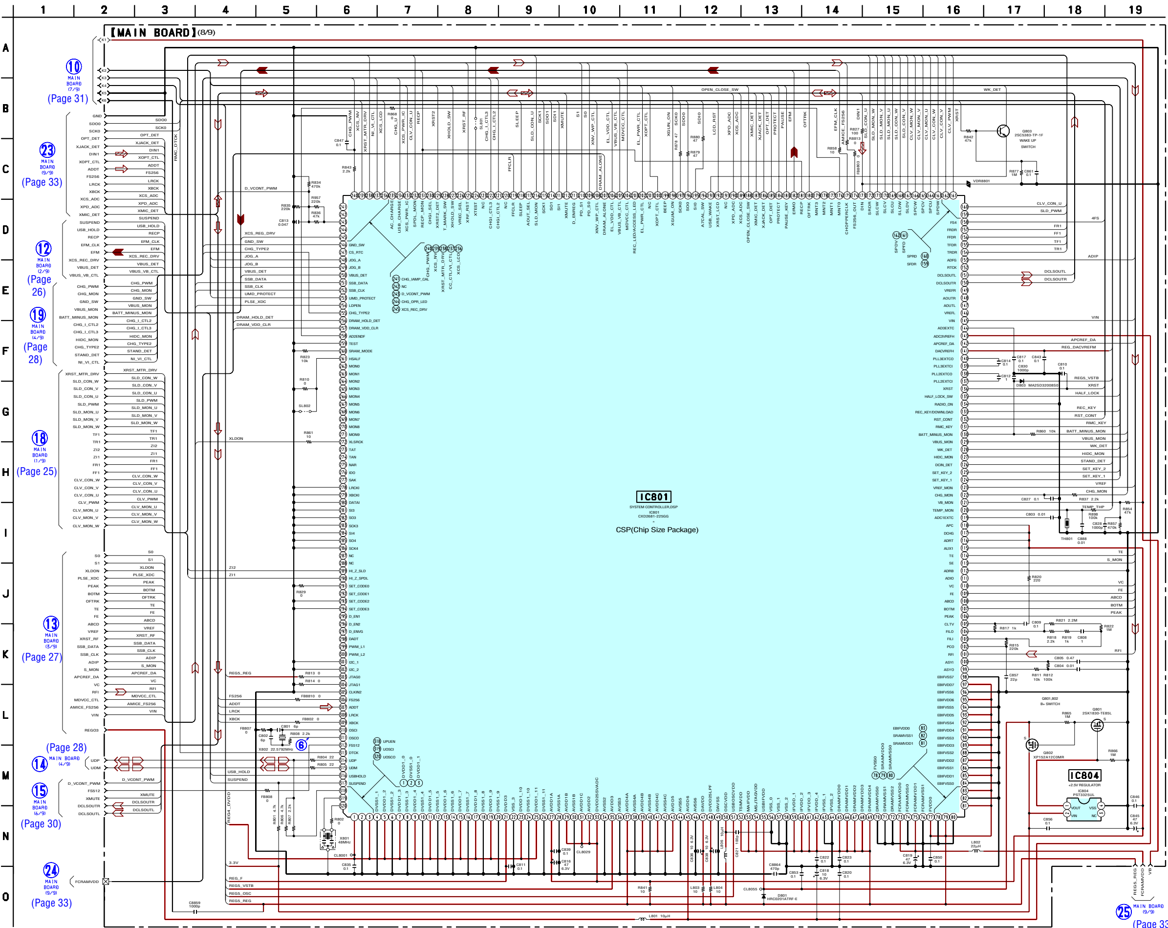
6-11. SCHEMATIC DIAGRAM – MAIN Board (8/9) – • See page 24 for Waveforms. • See page 41 for IC Pin Function Description.
